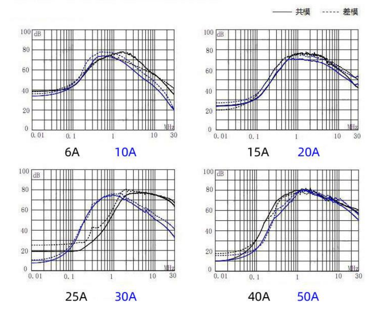
衰减值参考图：Typical Filter Attenuation
